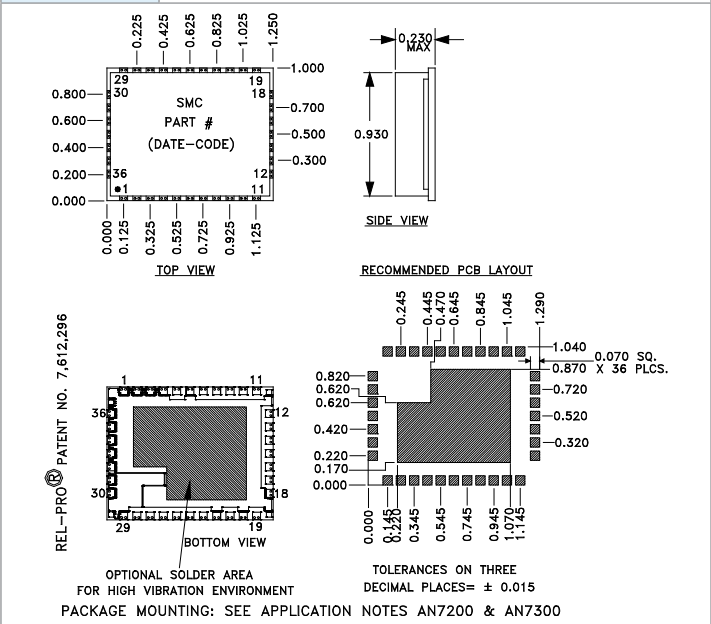
Package # 197LF
