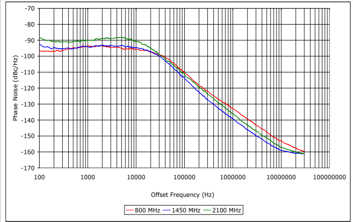
Phase Noise
